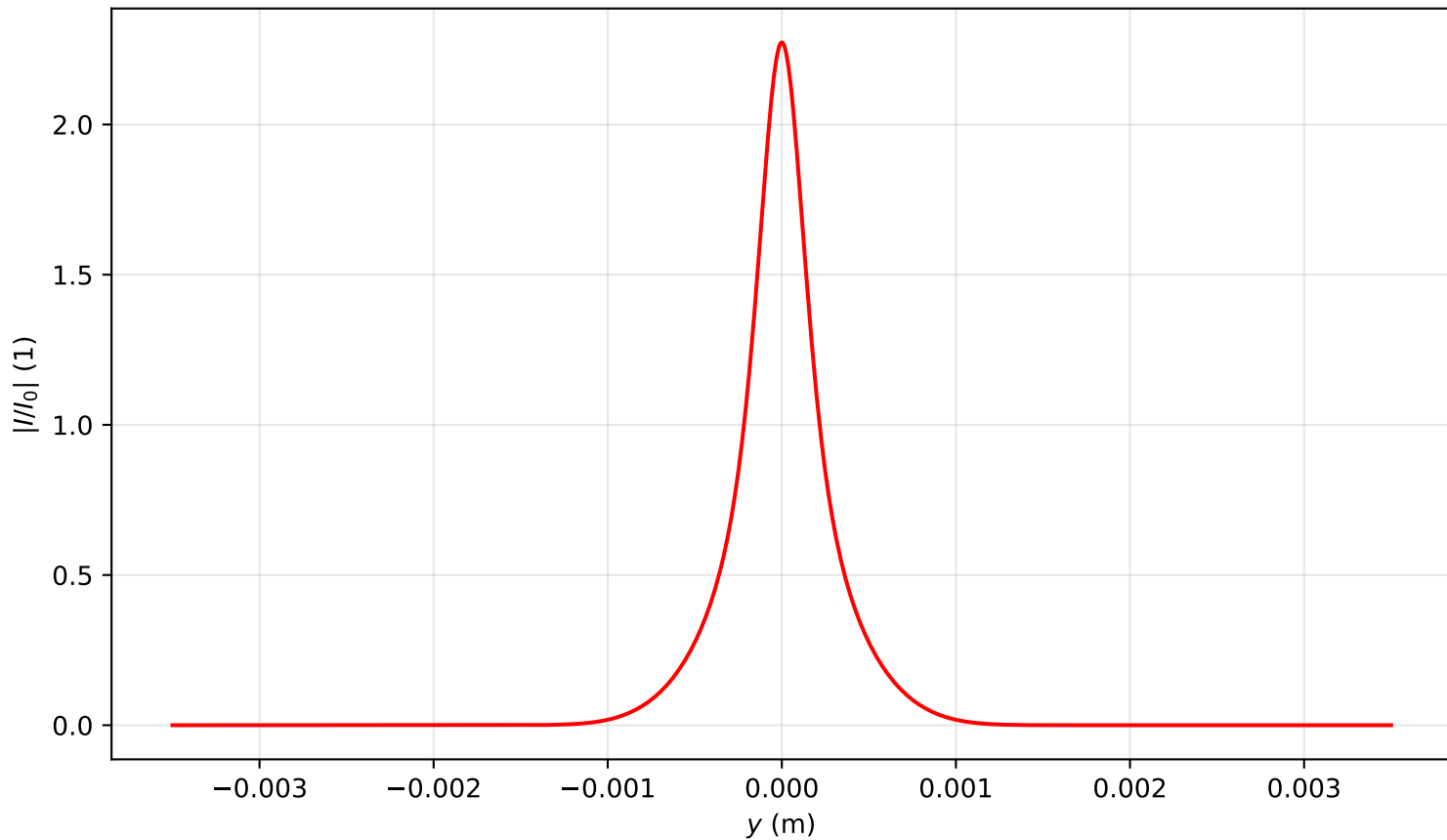
Intensity profile I(x = 0, y, z = 0.478)/I_0 , P_{in}=3.0P_{cr} , artificial time
